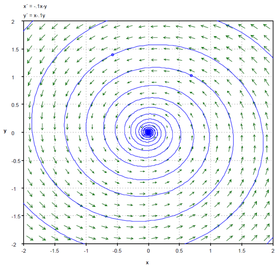
Slow spiral in: complex eigenvalues with small negative real part
