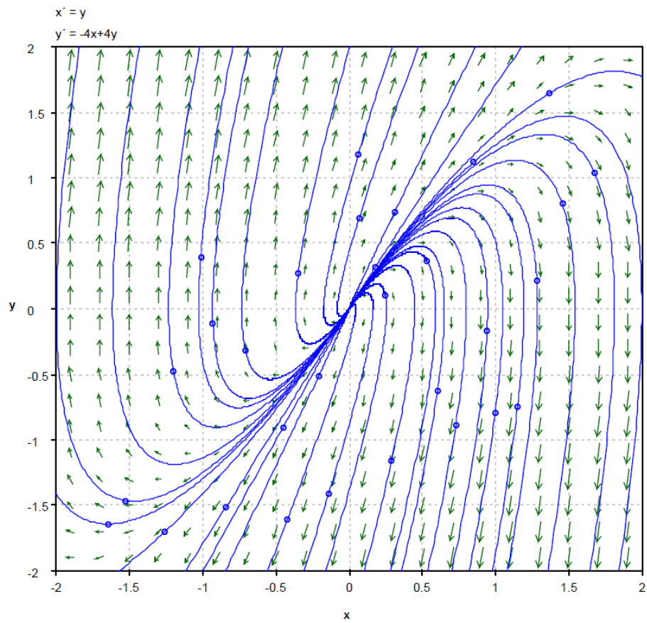
Unstable node: One repeated positive eigenvalue, not diagonalizable
