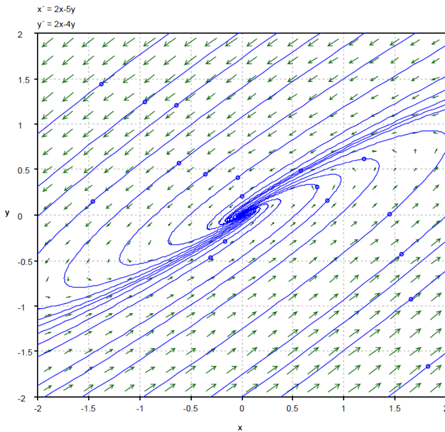
Counterclockwise Spiral In: Complex eigenvalues with negative real part
