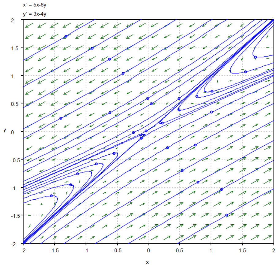
Real eigenvalues: One positive, one negative
